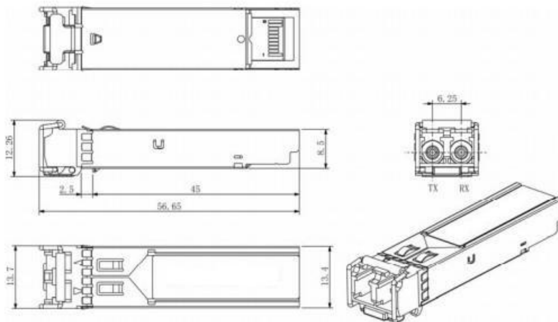
Mechanical Drawing
