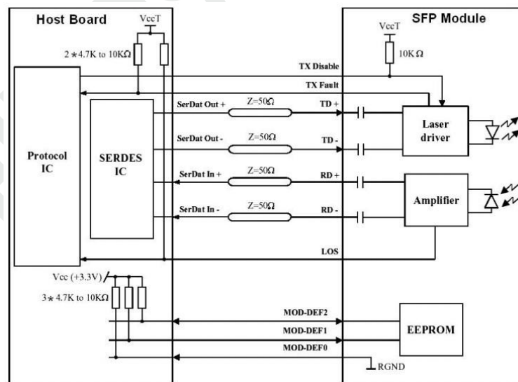
SFP Host Recommended Circuit
