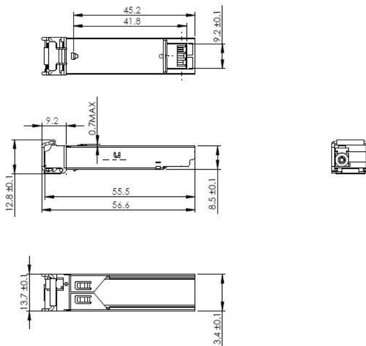
Mechanical Drawing
