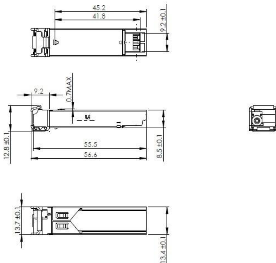
Mechanical Drawing
